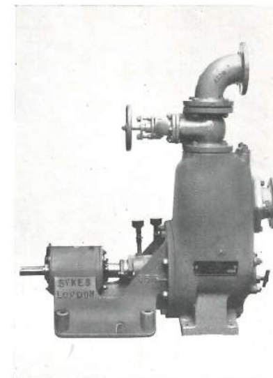
Latest type of Self-priming Centrifugal Pump.
