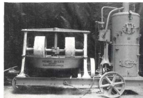
Portable Mortar Mill.
